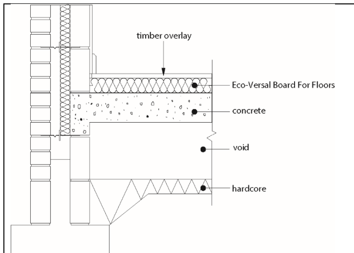
Figure 4 Suspended concrete ground floor — timber overlay
