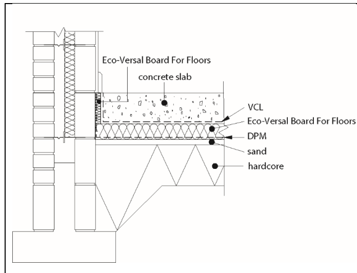
Figure 3 Ground-bearing concrete — slab overlay
