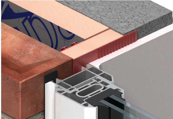
Figure 8: Kingspan Kooltherm® Cavity Closer at a normal reveal
