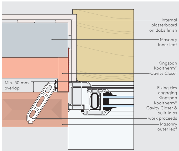
Figure 4: Jamb detail incorporating Kingspan Kooltherm® Cavity Closer at a normal reveal
