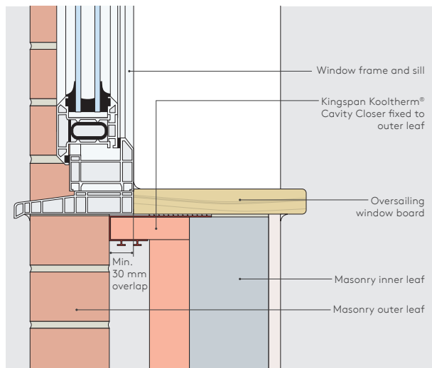
Figure 5: Sill detail incorporating Kingspan Kooltherm® Cavity Closer at a normal reveal
