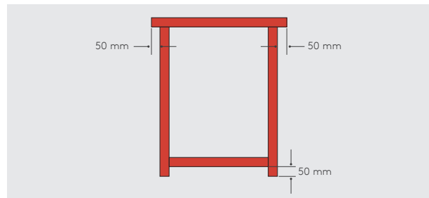
Figure 10: Kingspan Kooltherm® Cavity Closer sill, jamb & head sections
