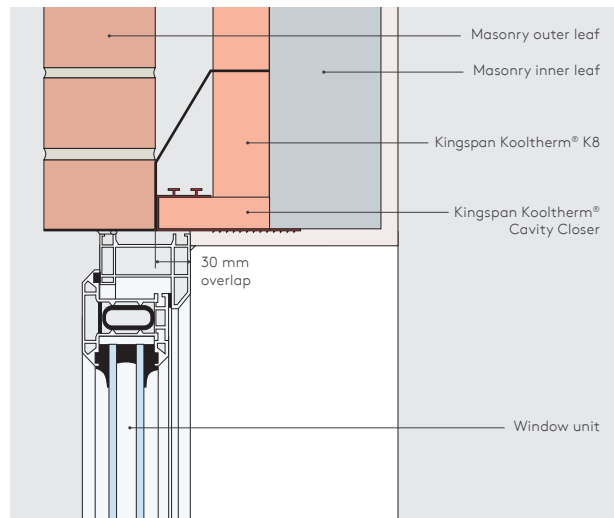
Figure 7: Head detail incorporating Kingspan Kooltherm® Cavity Closer
