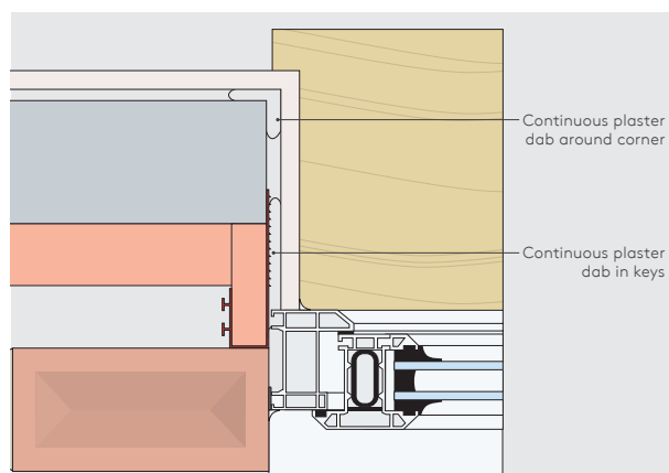
Figure 11: Kingspan Kooltherm® Cavity Closer with continuous plaster dab in fins
