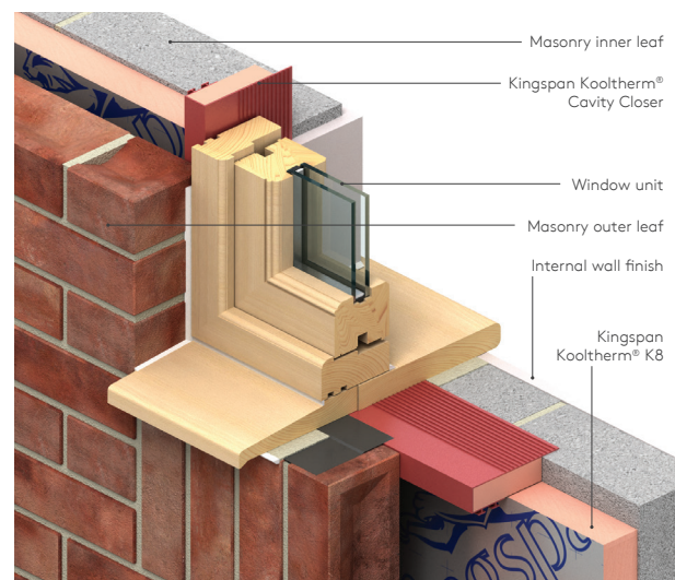
Figure 2: Kingspan Kooltherm® Cavity Closer in a masonry cavity wall construction with Kingspan Kooltherm® K8 Cavity Board
