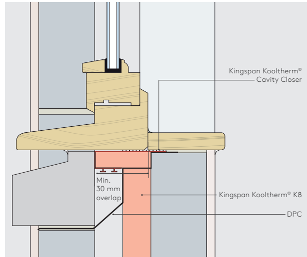
Figure 6: Sill detail incorporating Kingspan Kooltherm® Cavity Closer
