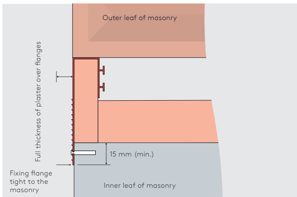
Figure 9: Basic installation principles
