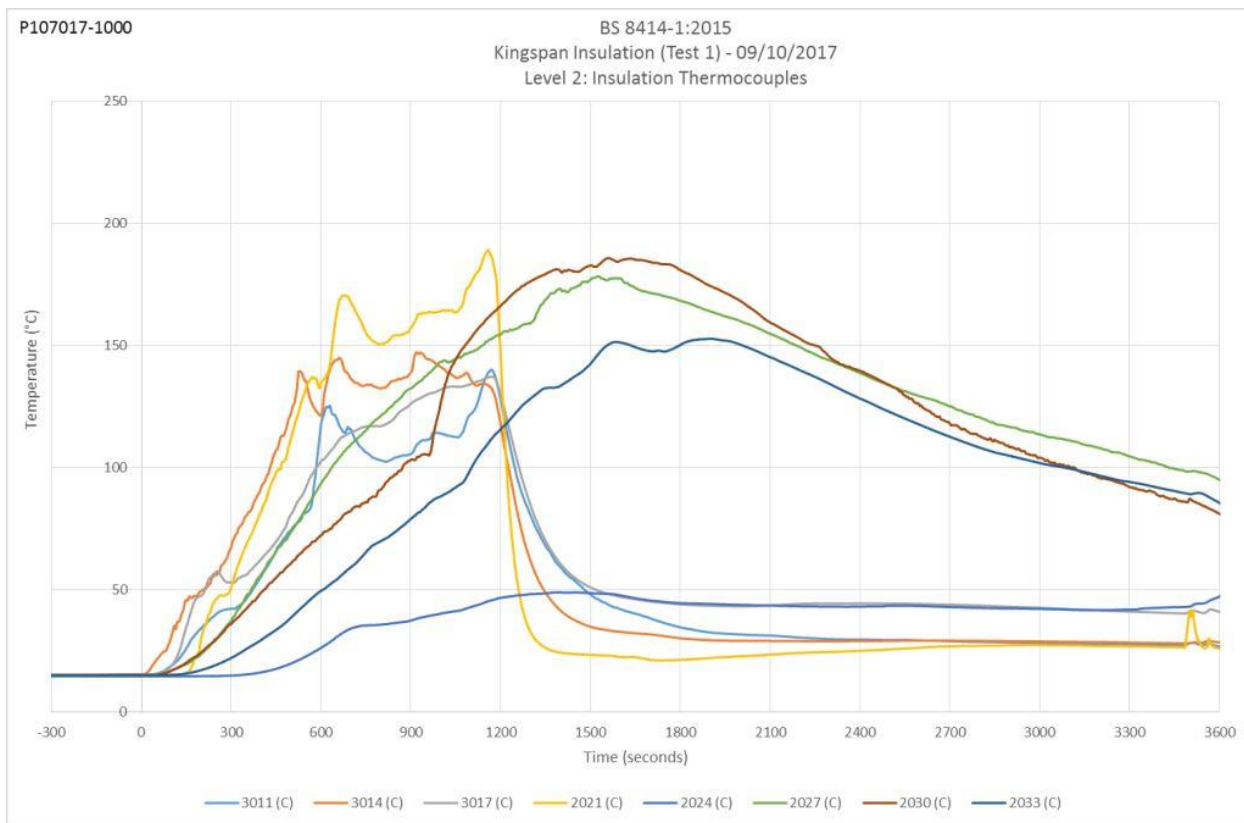
Figure 13. Level 2 insulation thermocouples. ts= 1 minute 55 seconds after ignition of the crib.
