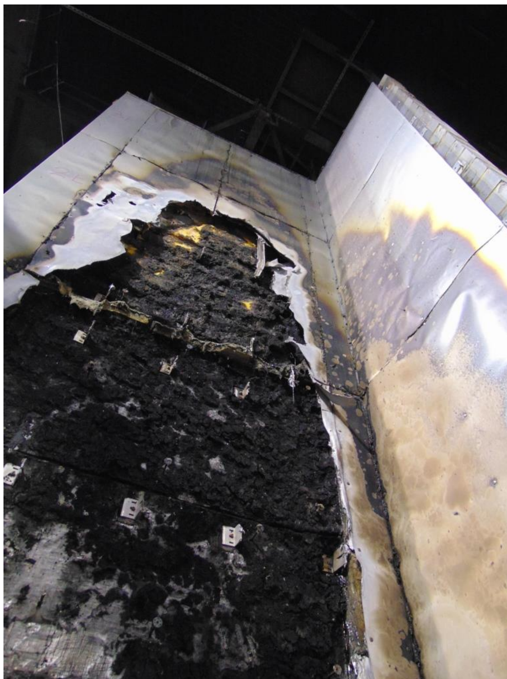
Figure 15. Post-test photo of exposed insulation on the main wall.
