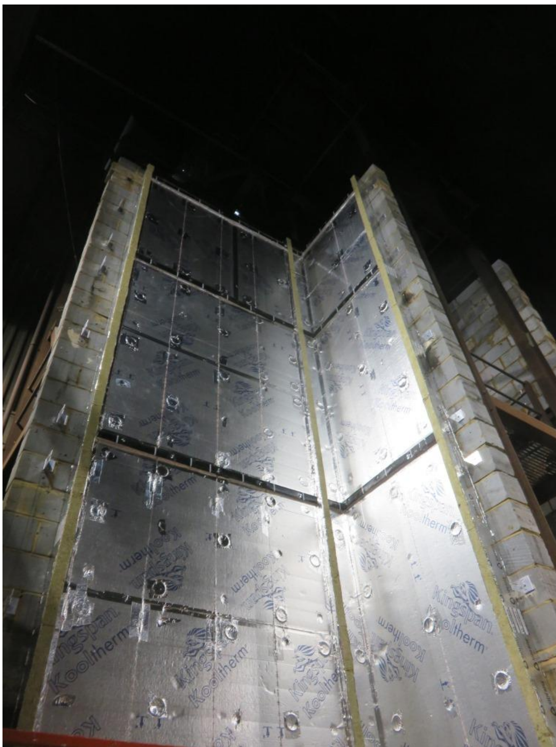
Figure 5. Partial installation of Siderise RH25G 90/30 horizontal open state cavity barriers and Kingspan Kooltherm K15 insulation.
