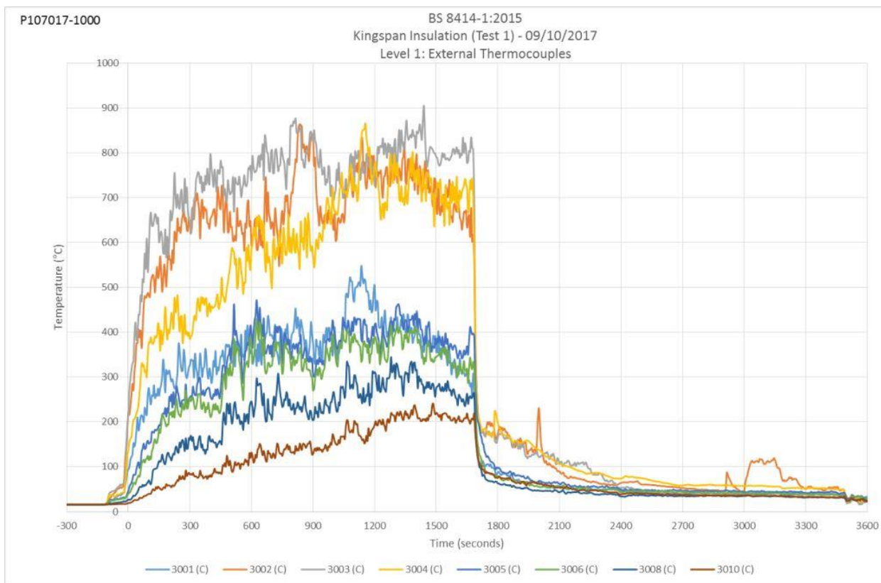
Figure 10. Level 1 external thermocouples. t_s = 1 minute 55 seconds after ignition of the crib.
