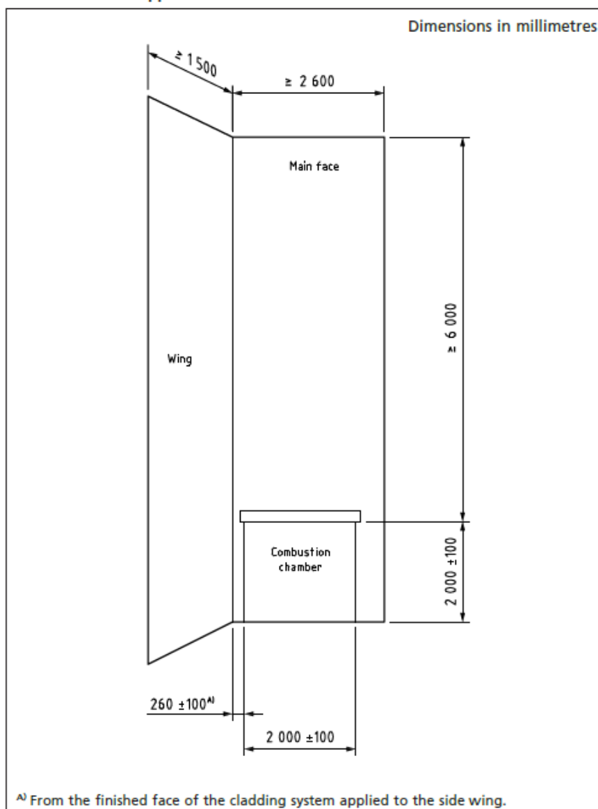
Figure 1 Schematic of test apparatus
