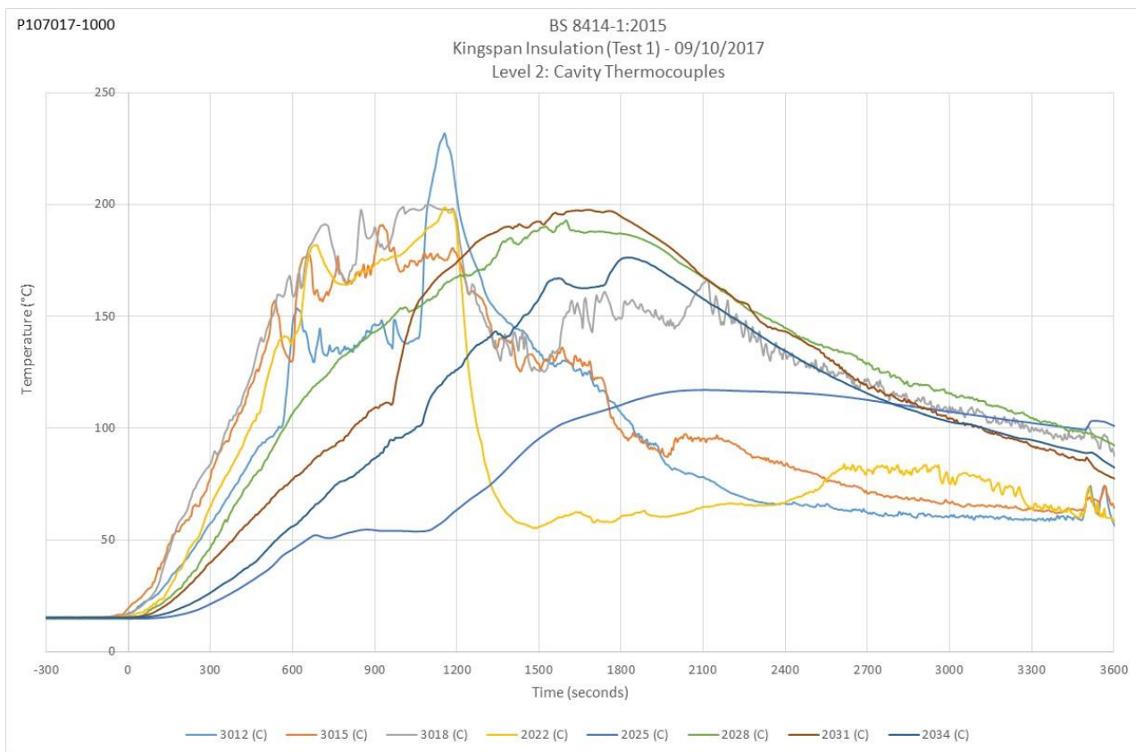
Figure 12. Level 2 cavity thermocouples.
