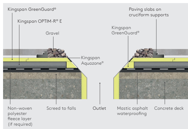
Figure 8 - Two level drainage
