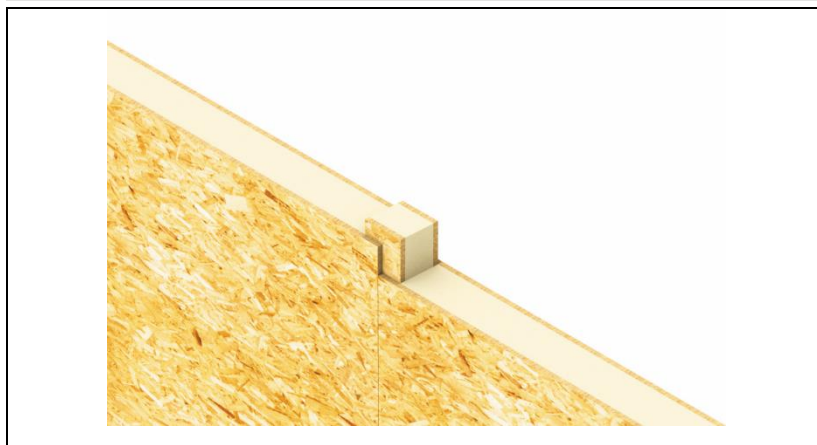
Figure 1 Cassette joint system
