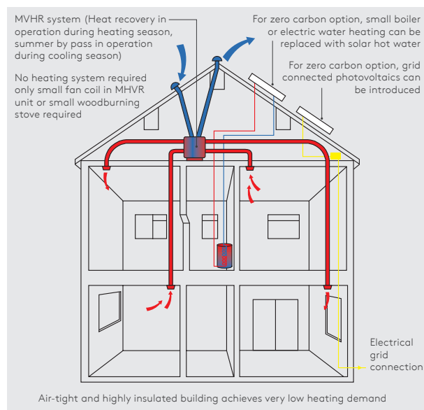
Figure 7: Heating systems in the Kingspan TEK® Building System
