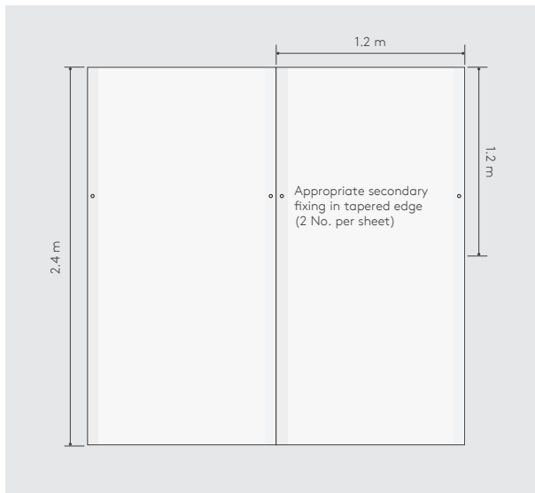
Figure 3: Appropriate secondary fixing pattern
