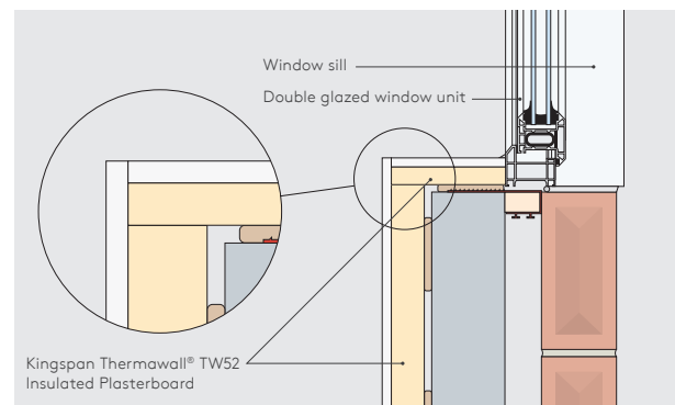
Figure 8: Insulated reveal and external corner
