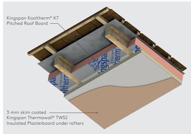
Figure 4: Mechanically fixed to timber rafters with Kingspan Kooltherm® K7 Pitched Roof Board between rafters
