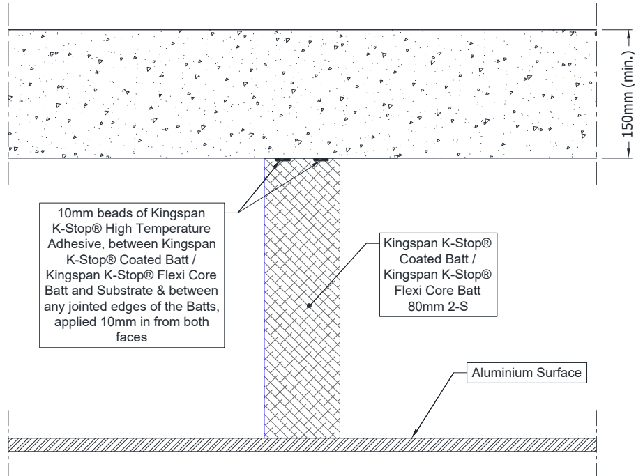
Construction details: Side View
