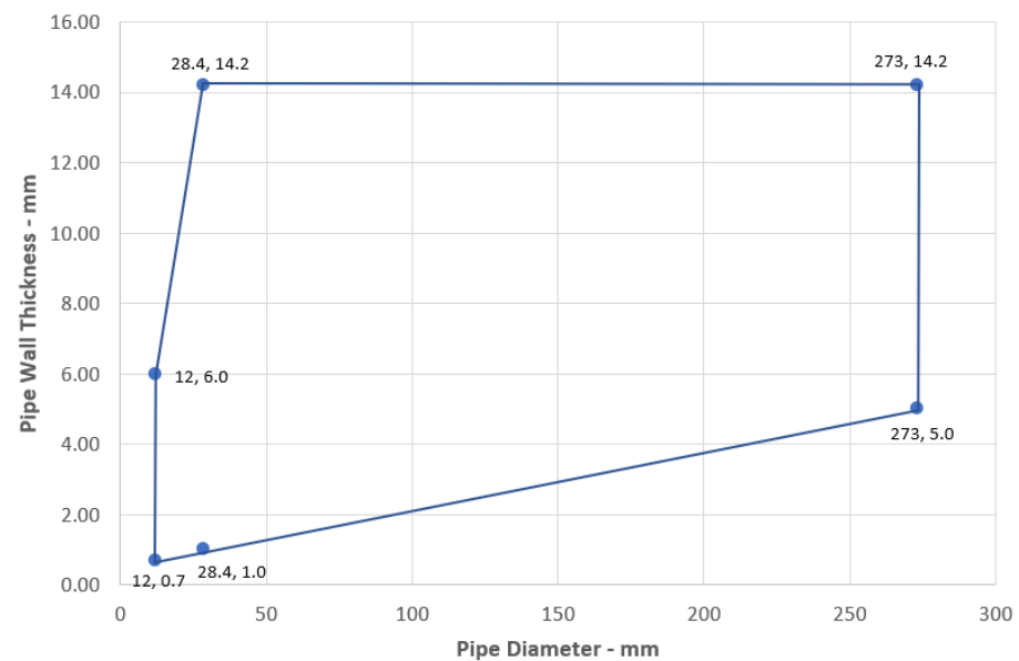
Mild or Stainless Steel Pipes with Stone or Glass Wool Insulation - C/C
