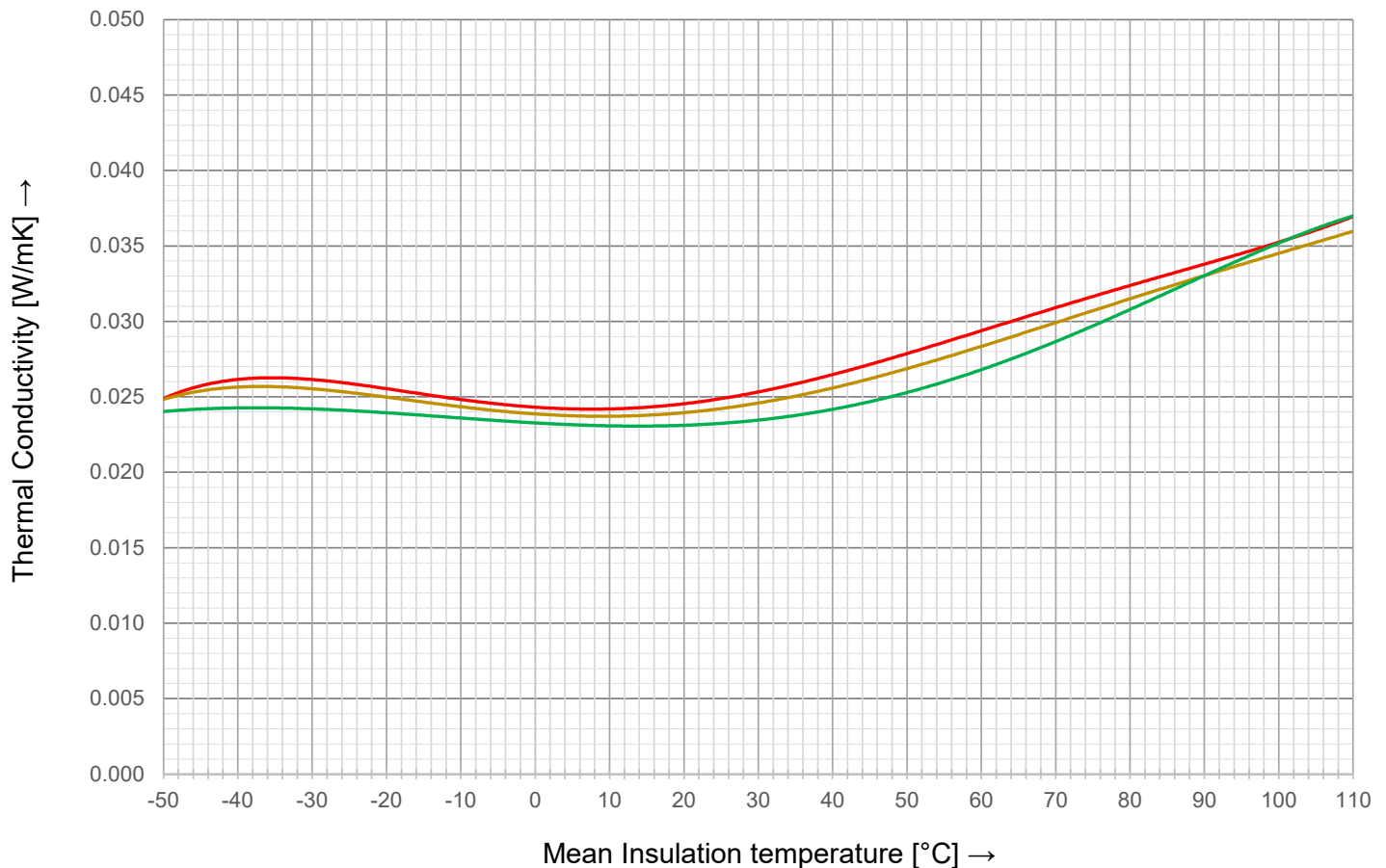
Thermal Conductivity Curve: Kooltherm® 37
