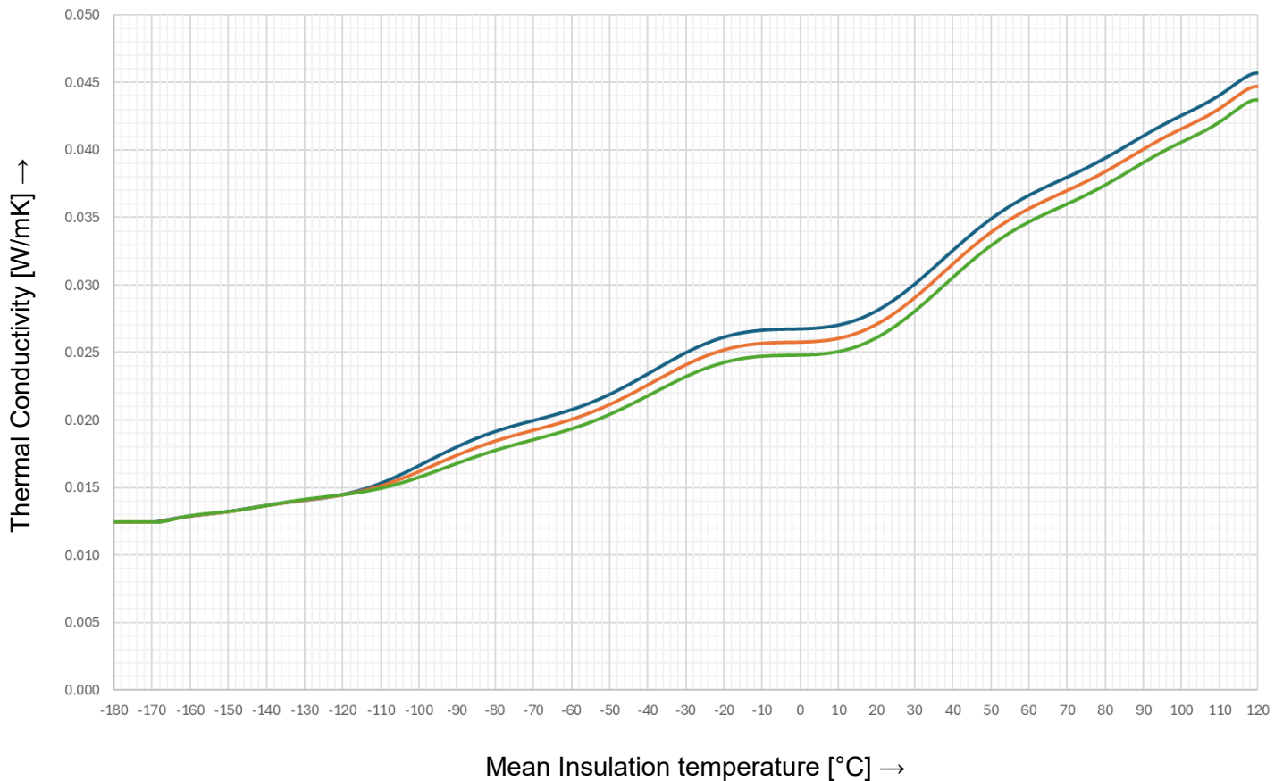
Thermal Conductivity Curve: Tarecpir M1-CR 42
